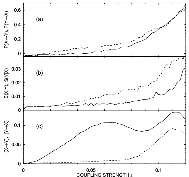
FIG. 3: (a) Cross-predictability P(X \rightarrow Y) (solid line) and P(Y \rightarrow X) (dashed line), (b) relative average distance of the mutual nearest neighbours S^{(k)}(\mathbf{Y}|\mathbf{X}) (solid line) and S^{(k)}(\mathbf{X}|\mathbf{Y}) (dashed line), and (c) coarse-grained transinformation rate i(X \rightarrow Y) (solid line) and i(Y \rightarrow X) (dashed line) for the unidirectionally coupled Rössler systems (5),(6), as functions of the coupling strength \epsilon .
