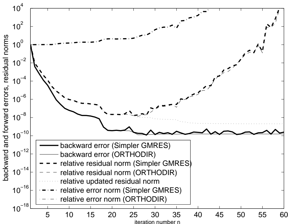
FIG. 3.1. The test problem FS1836 solved by Simpler GMRES and ORTHODIR: Normwise backward error \|b - Ax_n\| / (\|A\| \|x_n\|) (thick solid line - Simpler GMRES, thin solid line - ORTHODIR), relative true residual norm \|b - Ax_n\| / \|b\| (thick dashed line - Simpler GMRES, thin dashed line - ORTHODIR), relative norm of the updated residual \|r_n\| / \|b\| (dotted line), relative norms of the error \|x - x_n\| / \|x\| (thick dash-dotted line - Simpler GMRES, thin dash-dotted line - ORTHODIR).
