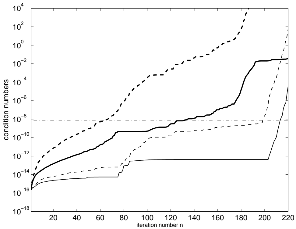
FIG. 3.6. The test problem STEAM1, condition numbers multiplied by unit roundoff u : \kappa(A) (dash-dotted line); \kappa(Z_n) (thick solid line) and \kappa(U_n) (thick dashed line) for Z_n = \begin{bmatrix} \frac{r_0}{\|r_0\|} \\ V_{n-1} \end{bmatrix} ; \kappa(Z_n) (thin solid line) and \kappa(U_n) (thin dashed line) for Z_n = \tilde{R}_n .
