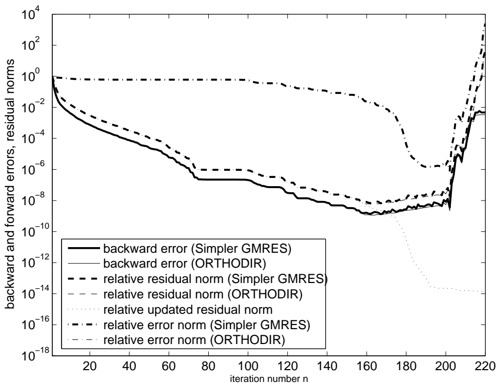
FIG. 3.4. The test problem STEAM1 solved by Simpler GMRES and ORTHODIR : Normwise backward error \|b - Ax_n\|/(\|A\|\|x_n\|) (thick solid line – Simpler GMRES , thin solid line – ORTHODIR ), relative true residual norm \|b - Ax_n\|/\|b\| (thick dashed line – Simpler GMRES , thin dashed line – ORTHODIR ), relative norm of the updated residual \|r_n\|/\|b\| (dotted line), relative norms of the error \|x - x_n\|/\|x\| (thick dash-dotted line – Simpler GMRES , thin dash-dotted line – ORTHODIR ).
